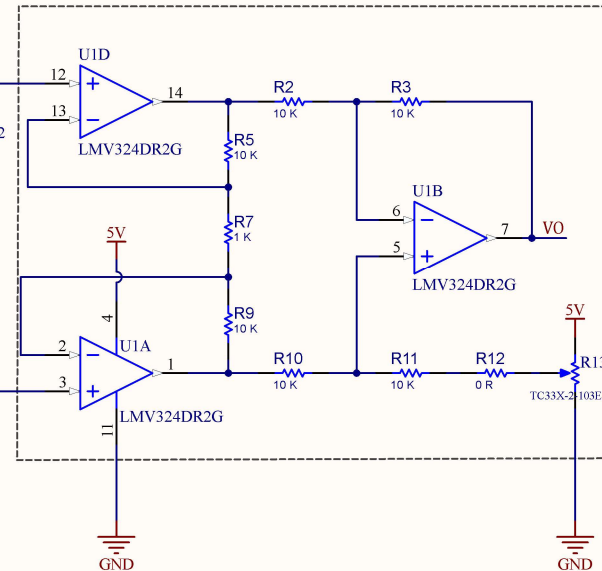
2SMPP-02 CIRCUIT
