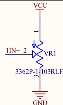
SENSITIVITY POT
