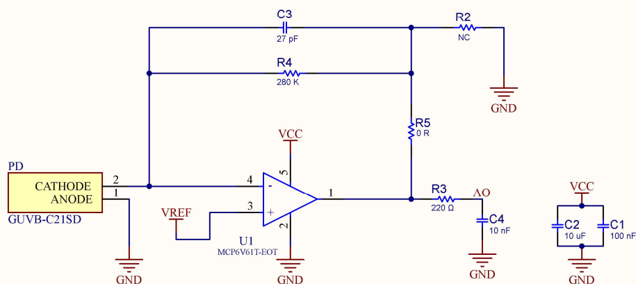
PHOTODIODE CIRCUIT
