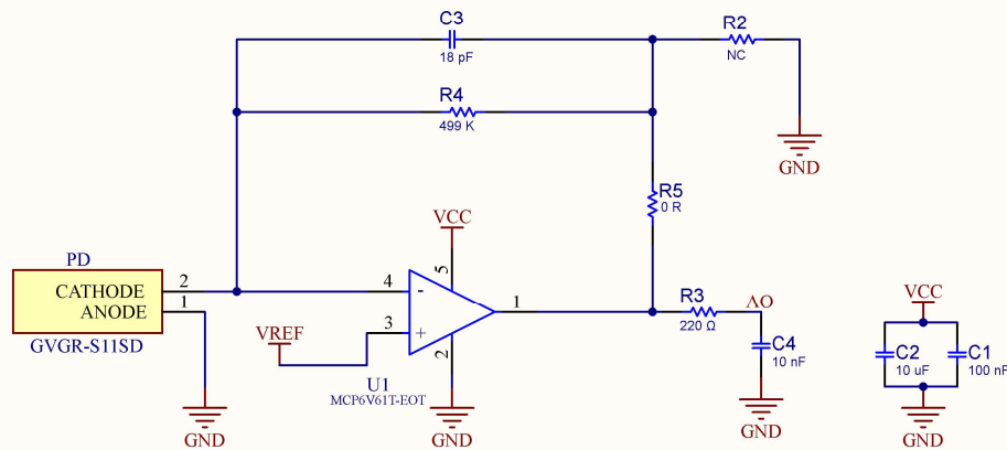
PHOTODIODE CIRCUIT
