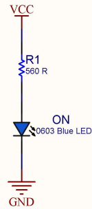
POWER LED
