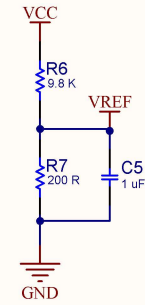
REFERENCE VOLTAGE
