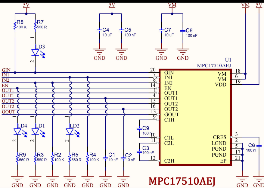
GATE DRIVER
