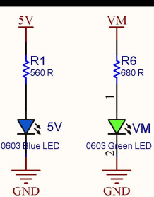
POWER LED
