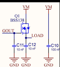
GATE DRIVER
