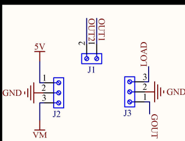
TERMINALS
