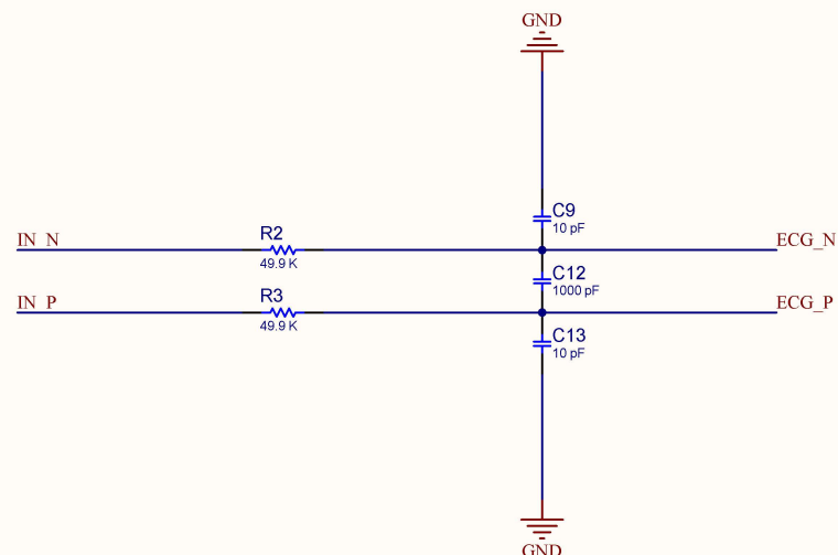
INPUT ECG SIGNALS
