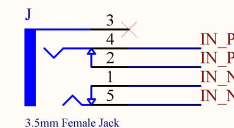
3.5mm HEADPHONE JACK
