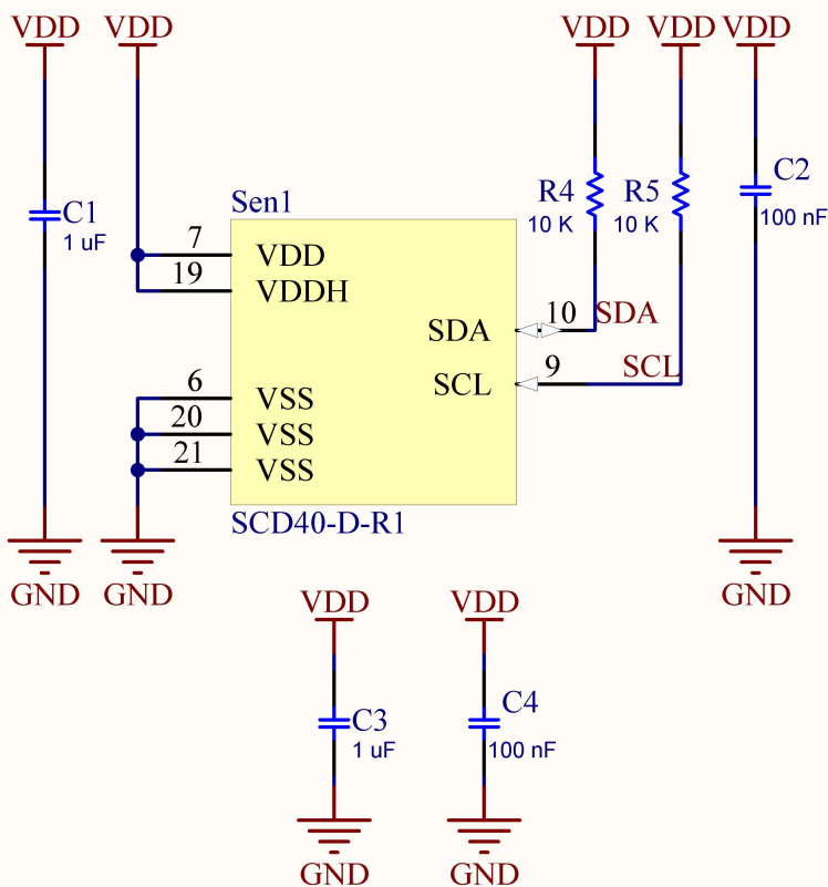
SCD40-D-R1 CIRCUIT
