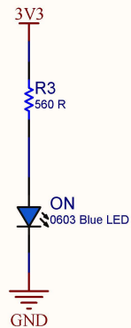
POWER LED
