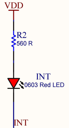
INTERRUPT LED
