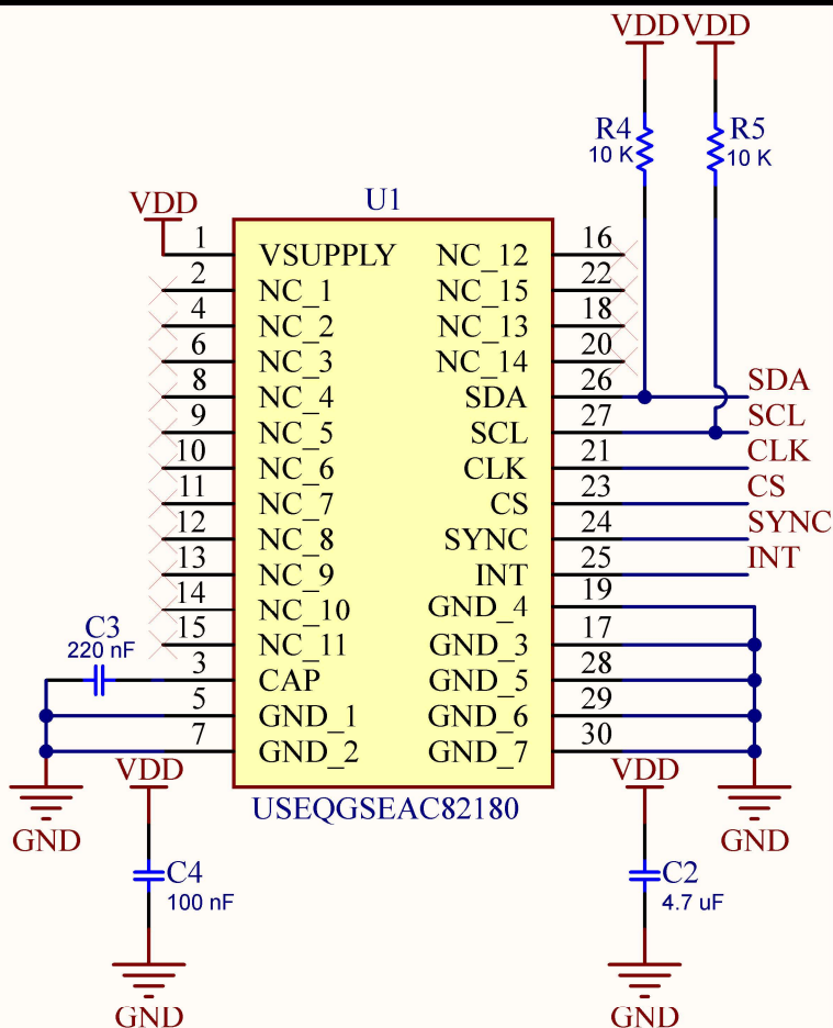
USEQGSEAC82180 CIRCUIT
