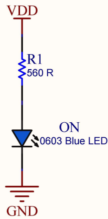
POWER LED
